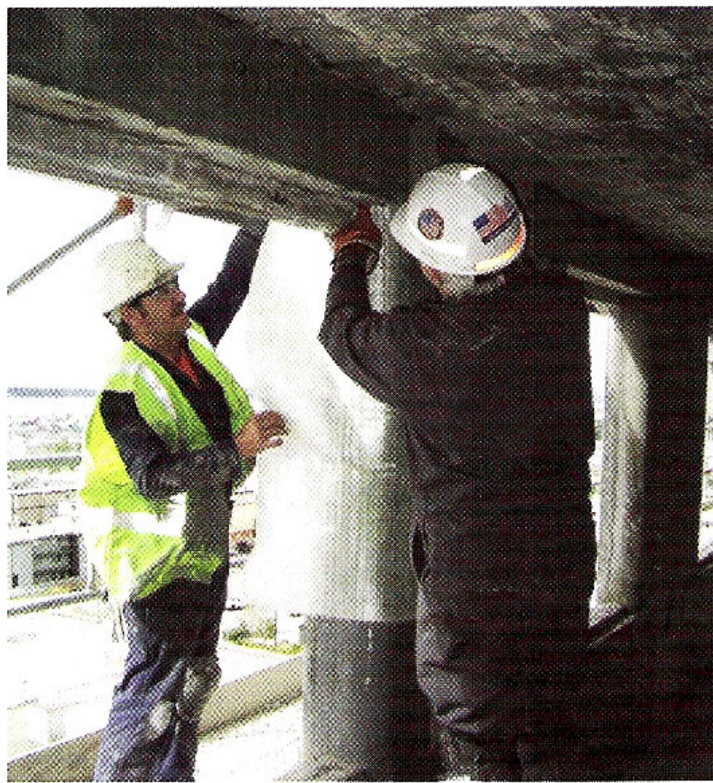
Fig. 5: Reinforcing boundary elements in shearwalls with GFRP
